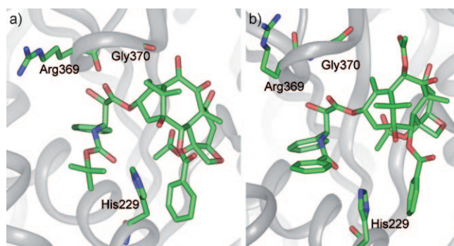
Figure 1. a) 1TUB and b) 1JFF.
