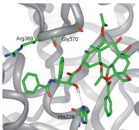
Figure 5. REDOR-taxol in 1TUB.
