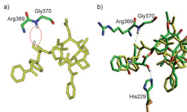
Figure 8. a) T-taxol-1JFF structure as received; b) Overlay of the minimized REDOR-taxol-1JFF (green; H bond with His229) and T-taxol-1JFF (yellow; H bond with Gly370) structures. For clarity, only heavy atoms and C2'-OH of Taxol and a few nearby residues are shown.
