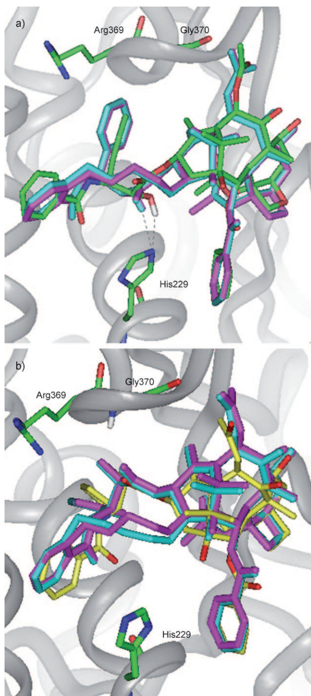
Figure 13. a) Overlay of the REDOR-taxol (green) with “REDOR-2053” (blue) and “REDOR-2054” (magenta) structures; b) overlay of the T-taxol structure (yellow) with “T-2053” (blue) and “T-2054” (magenta) structures.
