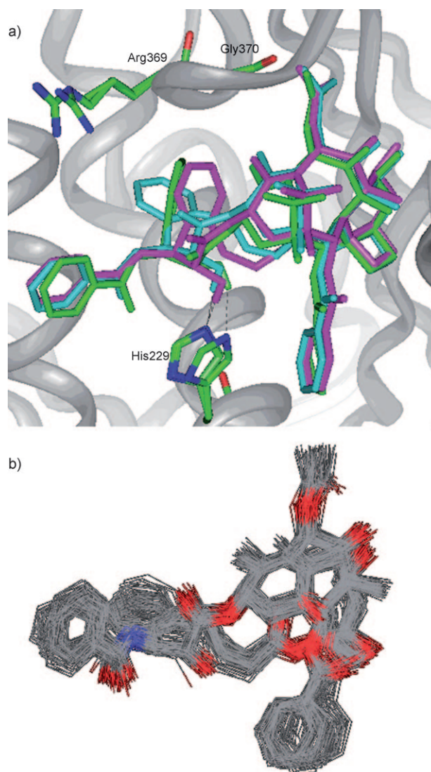
Figure 10. a) Overlay of the REDOR-taxol (green) with "REDOR-K1" (blue) and "REDOR-K2" (magenta) structures; b) MD simulation of the "REDOR-K2" in 1JFF. For clarity, only heavy atoms and C2'OH of taxoids and a few residues are shown.
