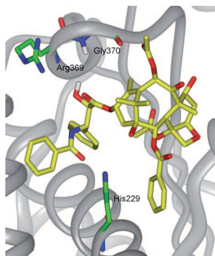
Figure 3. T-taxol in 1JFF. [37]
