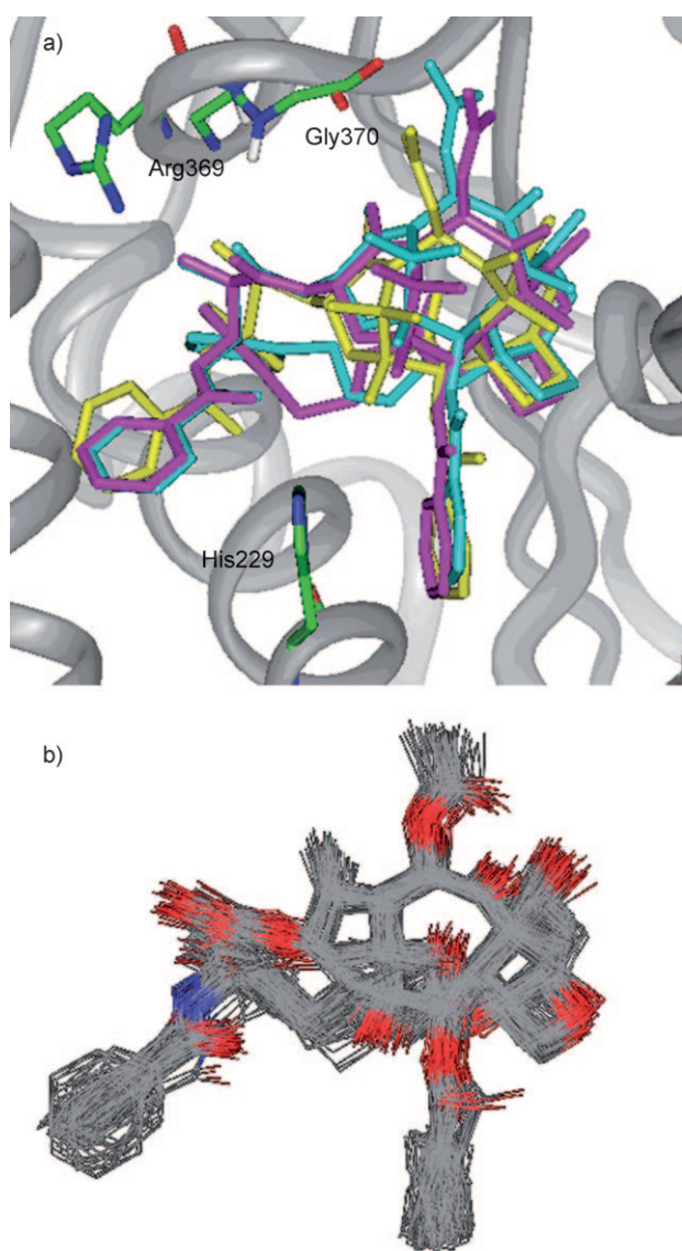
Figure 11. a) Overlay of the T-taxol structure (yellow) with "T-K1" (blue) and "T-K2" (magenta) structures; b) MD simulation of the "T-K2" in 1JFF. For clarity, only heavy atoms and C2'OH of taxoids and a few residues are shown.
