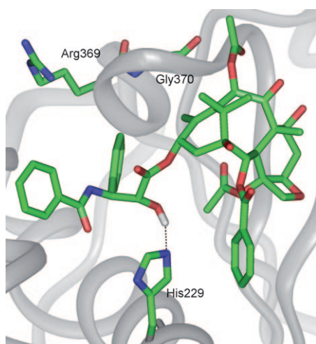
Figure 7. REDOR-taxol in 1JFF.
