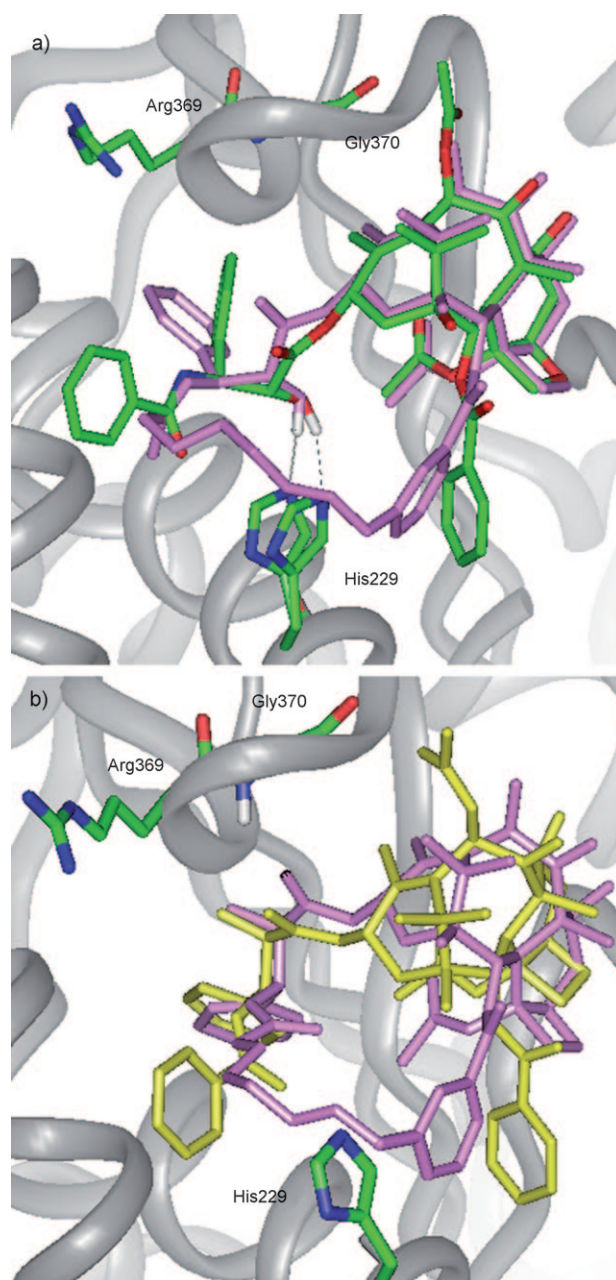
Figure 12. a) Overlay of the REDOR-taxol structure (green) with "REDOR-QT" (light magenta); b) overlay of the T-taxol structure (yellow) with "T-QT" (light magenta).
