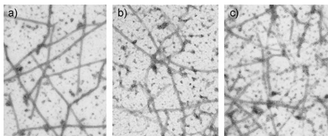
Figure 6. Electromicrographs of microtubule: a) GTP; b) paclitaxel; c) SB-T-2054.
